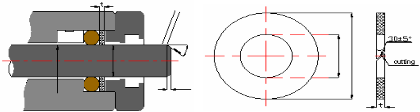
Teflon Back up Ring
