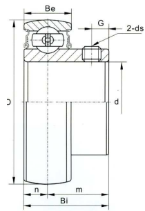
SB 200 (light-duty) Spherical O. D.
