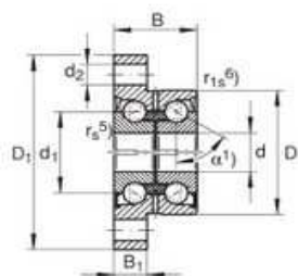
ZKLFA...2RS, ZKLFA...2Z
