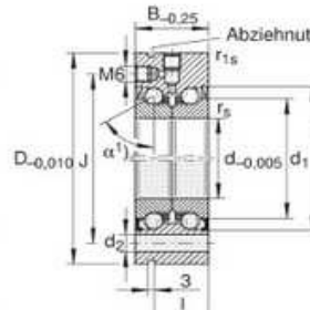
ZKLF...(d ≤ 50)
